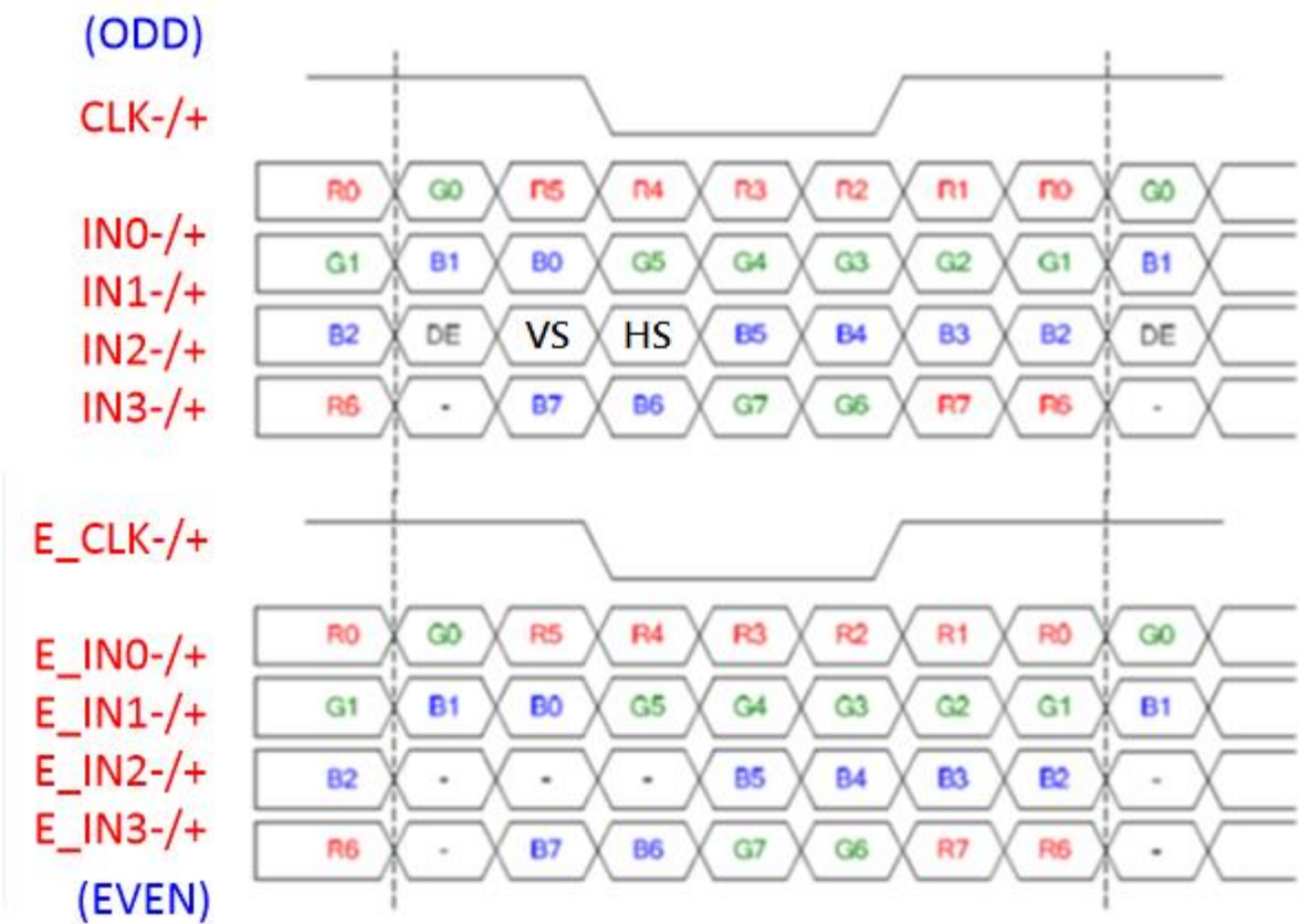
LVDS data mapping (VESA standard)
