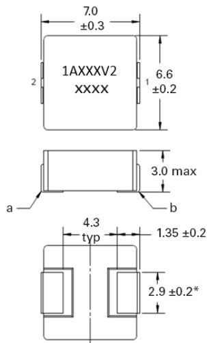
* HCM1A0703V2-R22-R (2.5 ±0.2)
