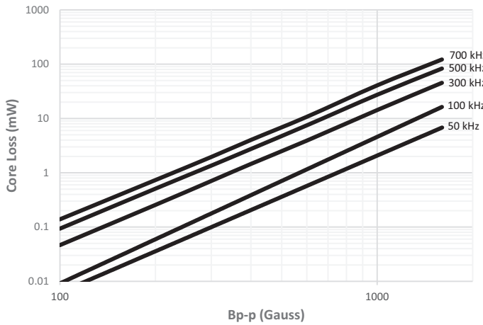
HCM1A0703V2-6R8-R
