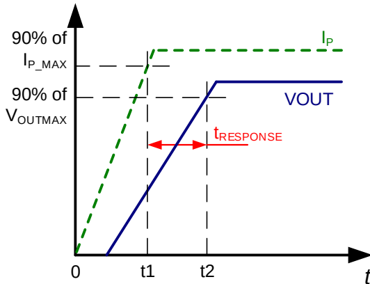
Figure 8: Response Time ( t_{RESPONSE} )
