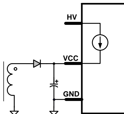
Figure 13: Start-up Circuit
